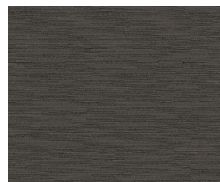
Java
