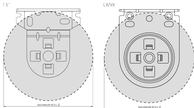
MAXIMUM ROLL SIZE CHART
