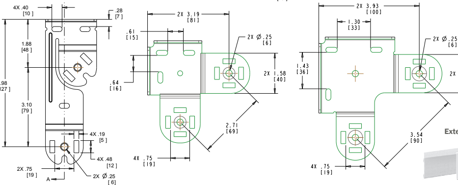
Dual Vertical Bracket (available in plated and white)
