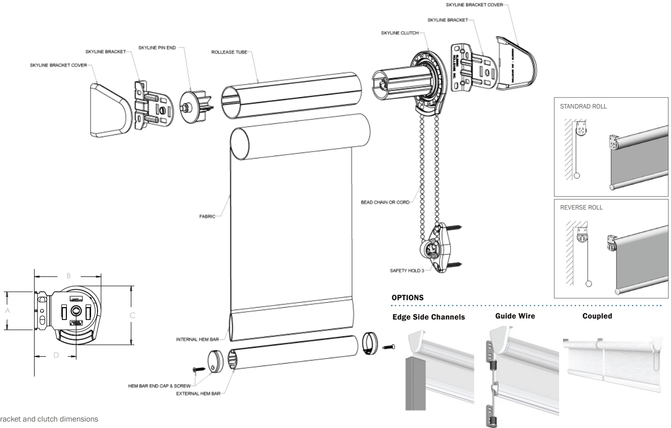
Skyline bracket and clutch dimensions
