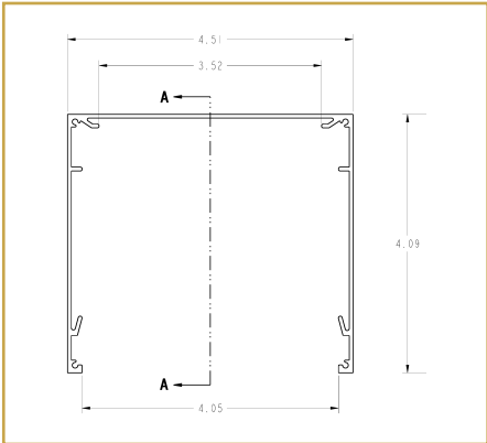
Legacy 4" 4.51" W x 4.09" H Single shade
