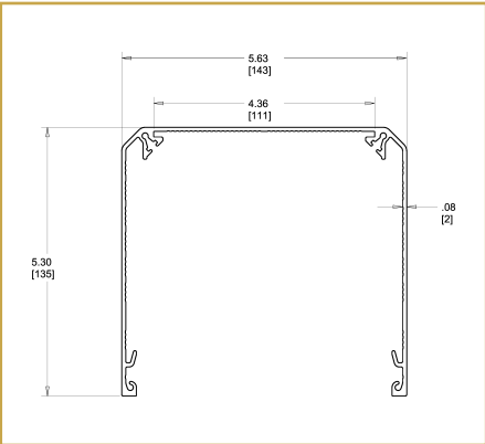
Legacy 5" 5.63" W x 5.30" H Single or dual shade
