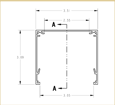
Legacy 3" 3.51" W x 3.09" H Single shade
