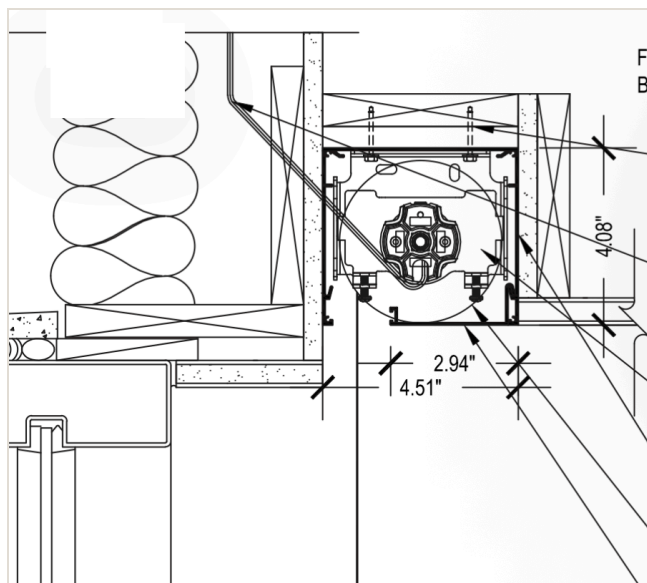
Ceiling-mount recessed pocket, AC motor — installation detail (Rollease Acmeda / Automate)
